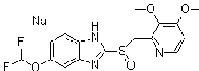
Figure 1. Pantaprazole Sodium (5-(Difluoromethoxy)-2-(((3,4-dimethoxy-2-yrindinyl)methyl) sulfinyl)-1H-benzimidazole sodium) used in present work
